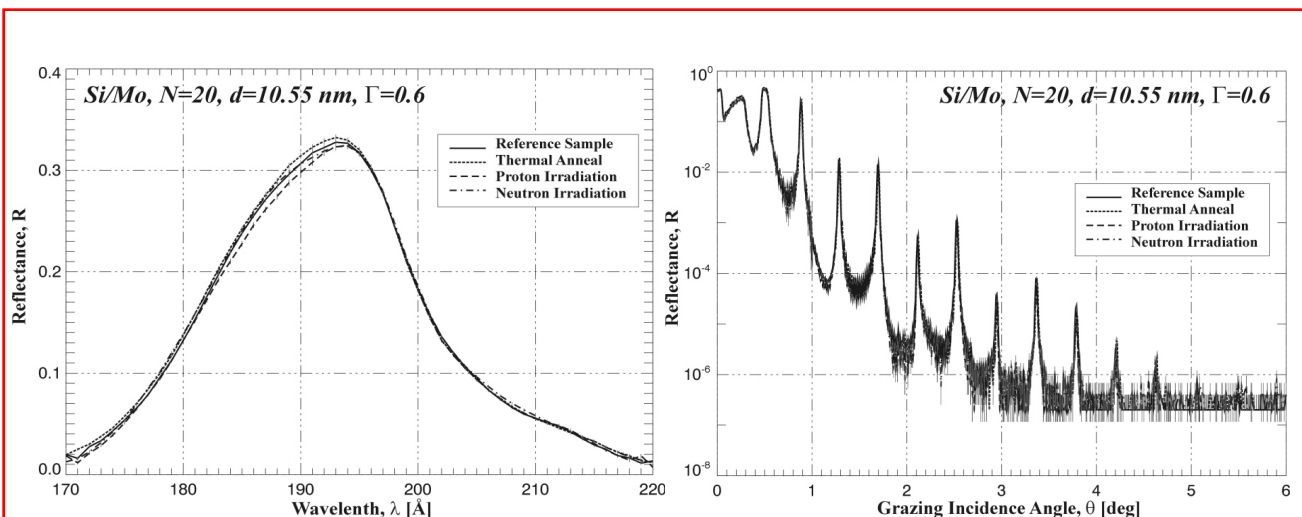
Figure 8 EUV and X-ray reflectance test on the Si/Mo multilayer sample reference, thermal annealing, proton and neutron test results superimposed.
